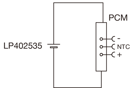
Circuit diagramm
